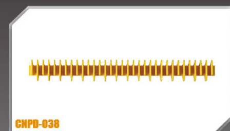
CNPB-038 产品参数 PRODUCT PARAMETERS Description: Front Shorter,33 uneven tooth,For aluminum step Suitable Brand: Thyssen
