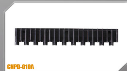
CNPD-010A 产品参数 PRODUCT PARAMETERS Description: Back Right, 22 uneven tooth, For stainless steel step Suitable Brand: Yungtay, Schindler, Guangri, LG, Toshiba, Hyundai
