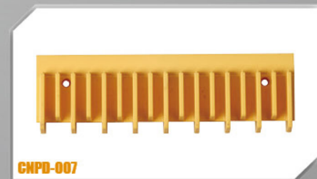
CNPD-007 产品参数 PRODUCT PARAMETERS Description: Front Center, 17 uneven tooth, For stainless steel step Suitable Brand: Yungtay, Schindler, Toshiba, SIEC, Fujitec
