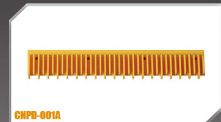
CNPD-001A 产品参数 PRODUCT PARAMETERS Description: Front, 38 uneven tooth, For S.S. Step Suitable Brand: XIZI OTIS
