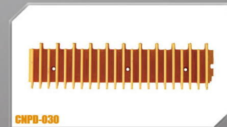
CNPD-030 产品参数 PRODUCT PARAMETERS Description: Front Center, 22 uneven tooth, For aluminum step Suitable Brand: Schindler
