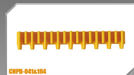
CNPB-041&184 产品参数 PRODUCT PARAMETERS Description: Front Shorter,17,For aluminum step Suitable Brand: Hyundai
